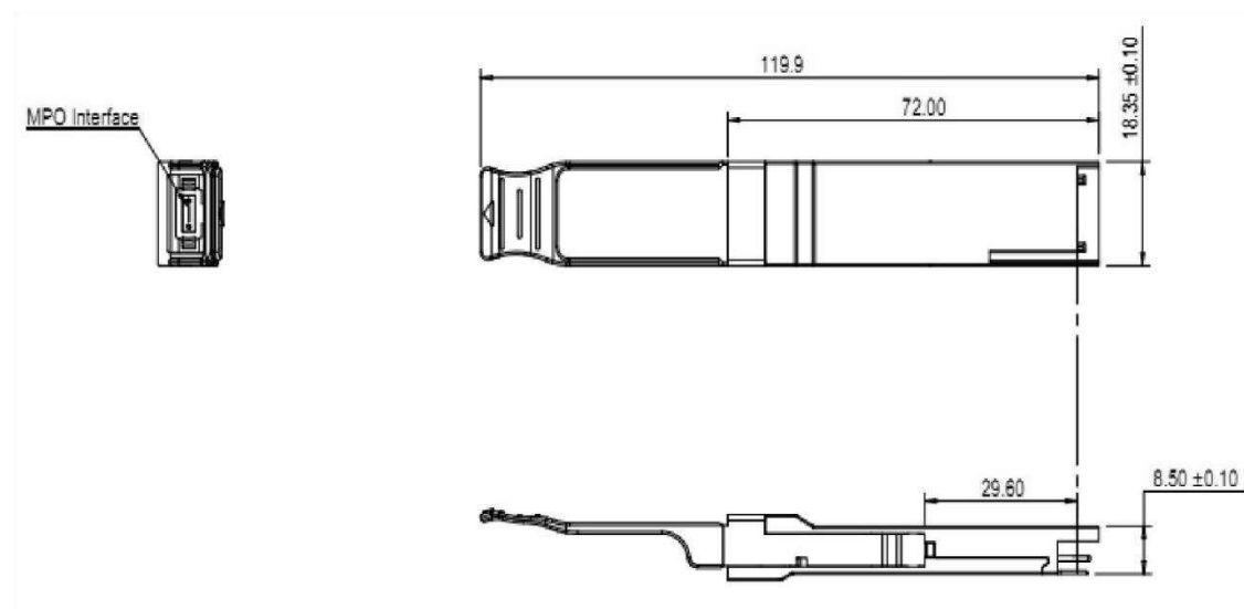
Figure 4 Package Dimensions
