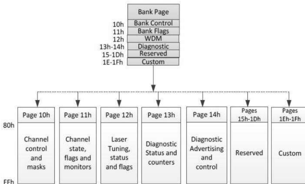
Figure 1 Digital Diagnostic Memory Map
