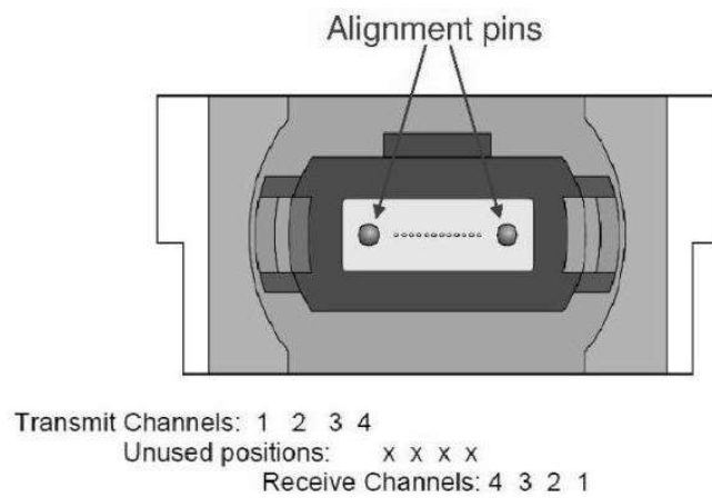
Figure 6 Optical lane sequence
