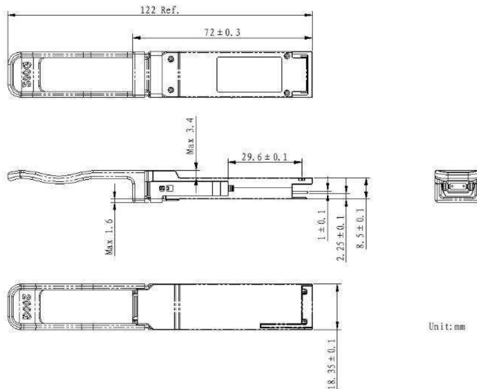
Figure 5 Package Dimensions
