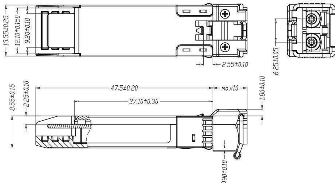
Figure 4 Package Dimensions
